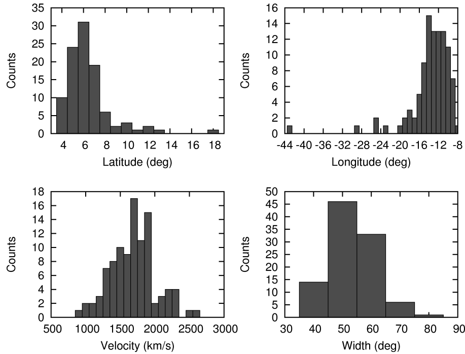
Figure 58. The input cone parameter distributions for the 3 May 1999 CME (event 1), derived from Coned Model version 1.3.
