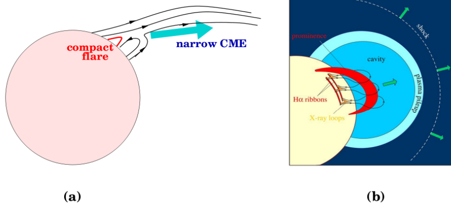
Figure 2. Diagrams of CME eruptions for narrow and normal CMEs: (a) Narrow CMEs, adapted from Chen [2011], (b) Normal CMEs, adapted from Forbes [2000].
