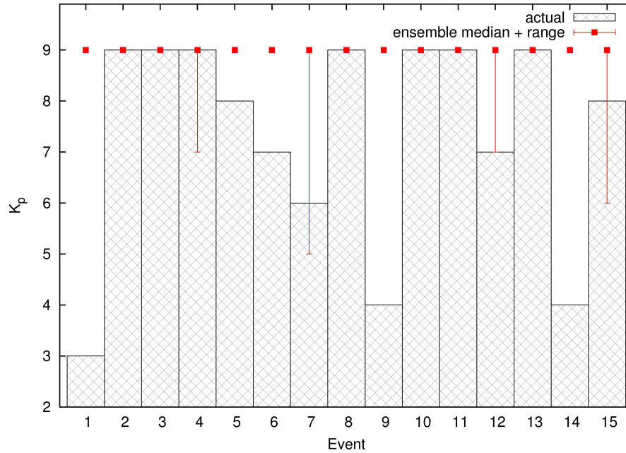
Figure 23. The median and range of the ensemble maximum K_p index forecast along with the actual maximum K_p index per event for the 15 CMEs.
