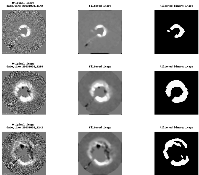
Figure 93. The filtered LASCOCO images for the 28 Oct 2003 CME (event 10), derived from Coned Model version 1.3.
