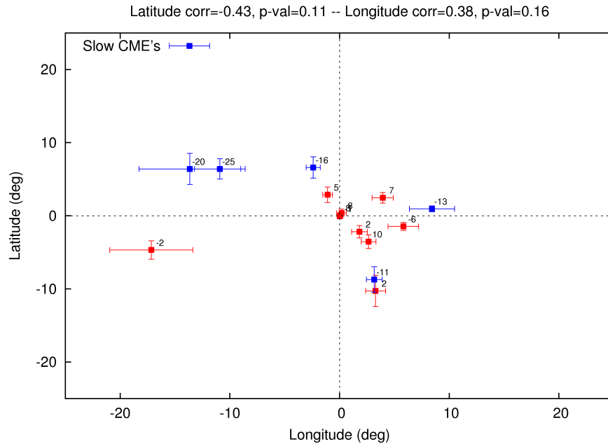
Figure 41. The Coned Model average latitude and longitude of the 15 CMEs with the forecast errors as the labels. The blue points are the slower CMEs with forecast errors less than -10 hours. The error bars are the standard deviations of the ensembles.
