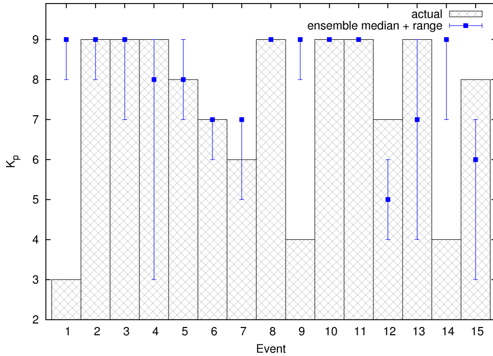
Figure 31. The median and range of the ensemble maximum K_p index along with the actual maximum K_p , per event, using Coned Model version 1.2.
